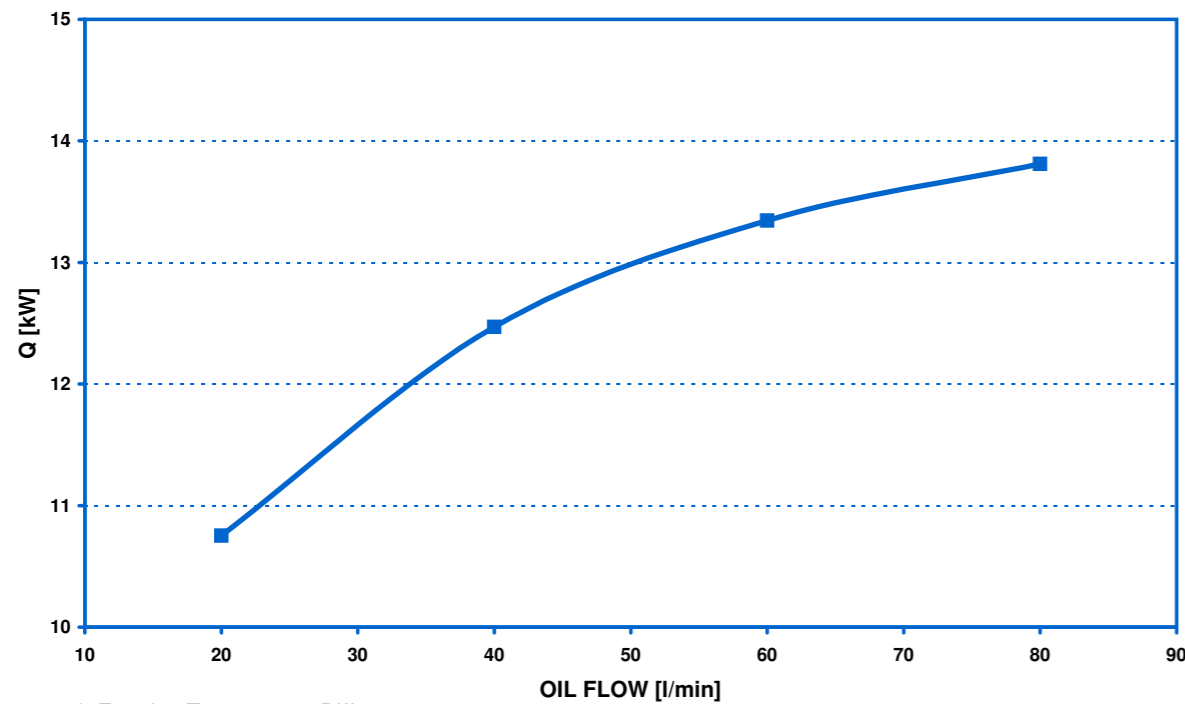
HEAT REJECTION AT ETD* 50 K AT 26 V
